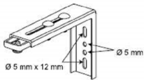
Double Adjustable Wall Mount Bracket - #1780910
