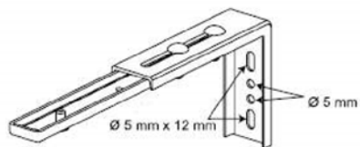
Double Adjustable Wall Mount Bracket - #1780910
